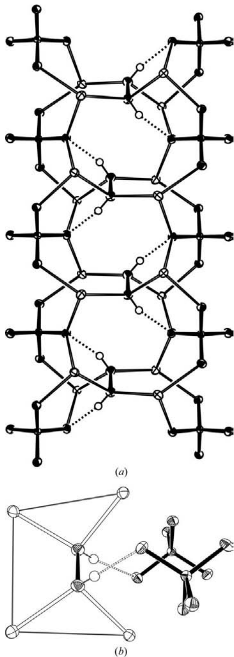
Figure 3 \text{H}_2\text{O}_2 environment in \text{Na}_9[\text{SO}_4]_4\text{X}\cdot 2\text{H}_2\text{O}_2 . Projections down (a) a and (b) c . The c axis is directed up the page in the top view.
